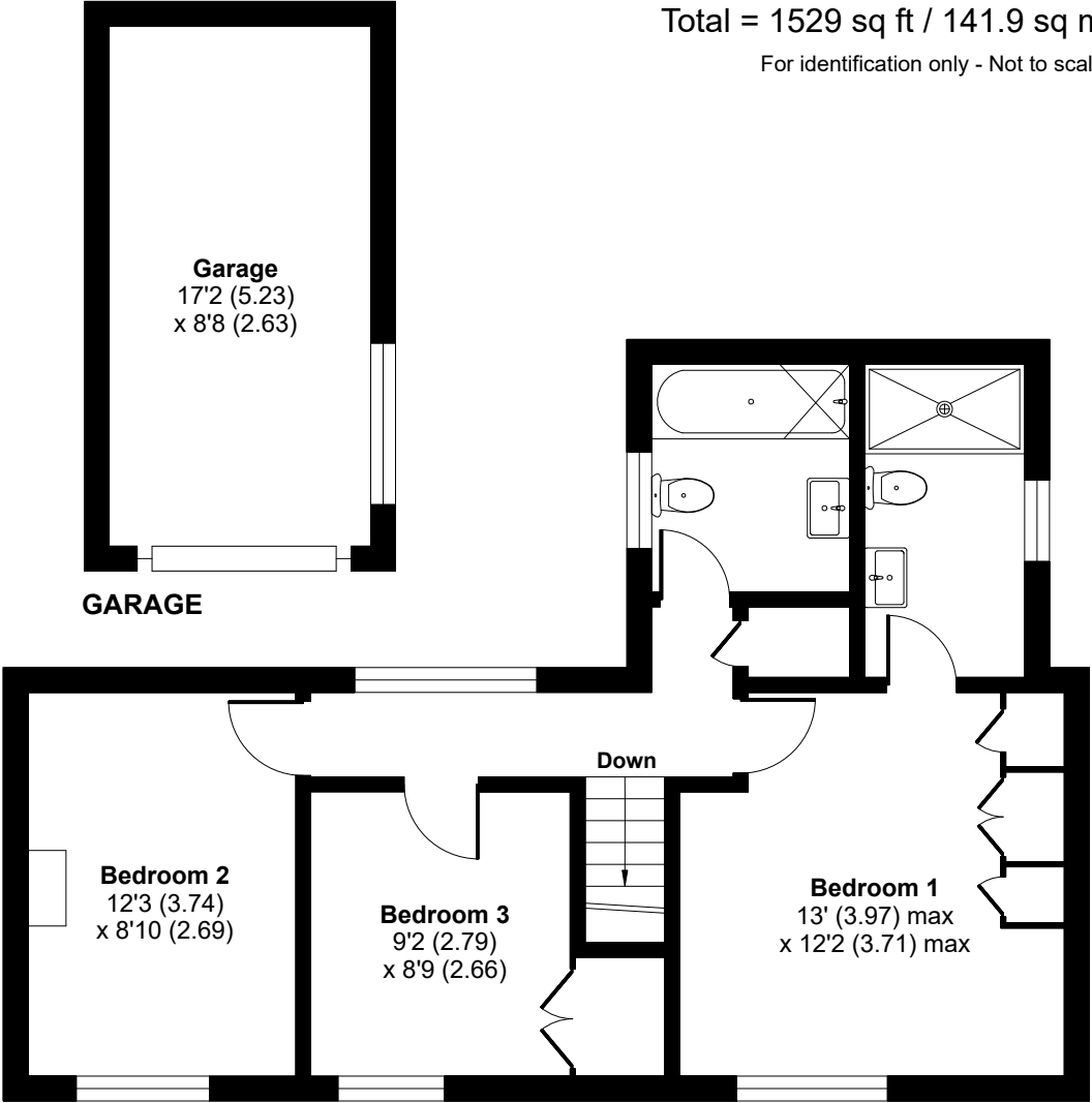
FIRST FLOOR
